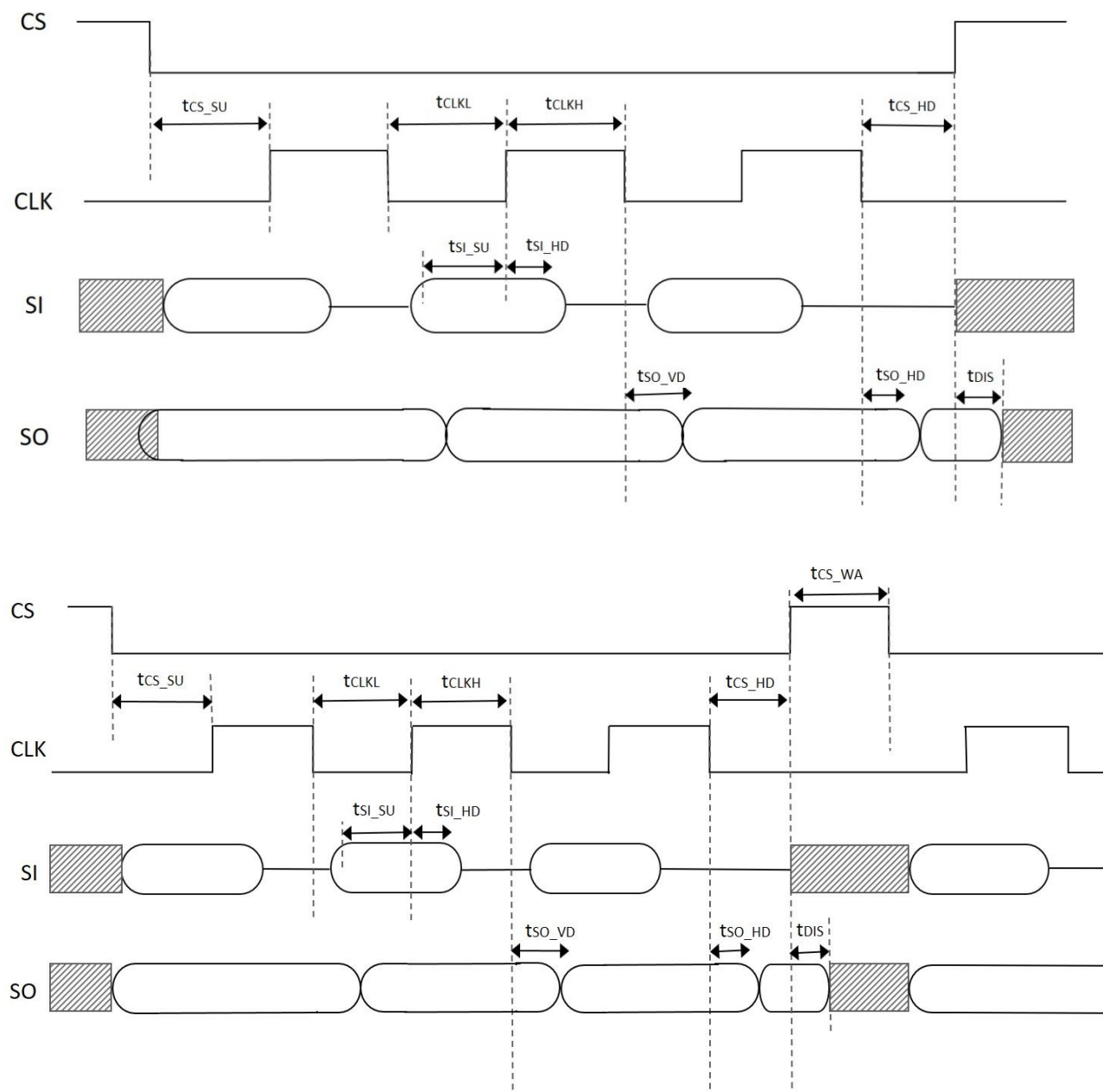
Figure 3-3 SPI Sequence
